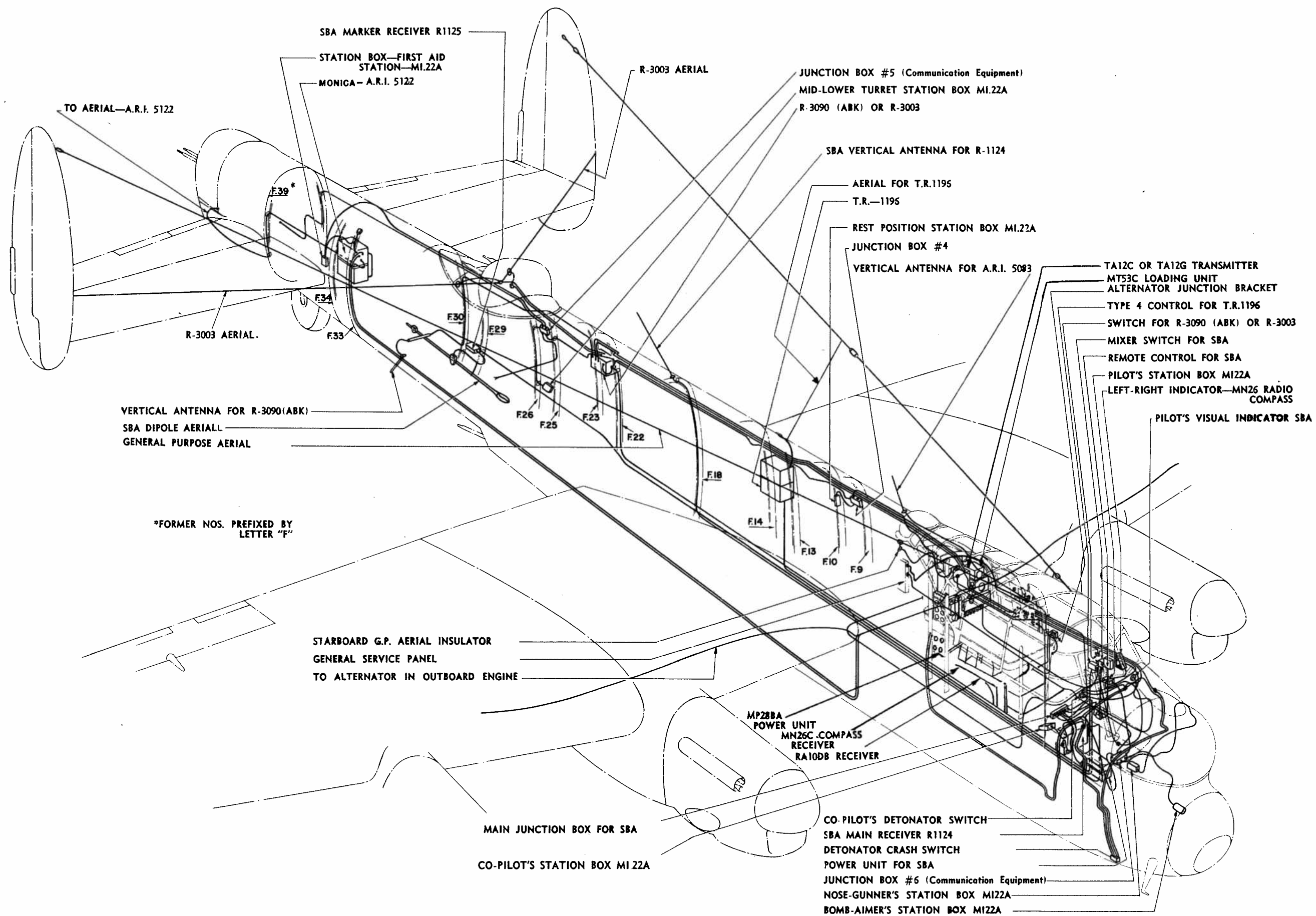
FIGURE 1—OUTLINE VIEW
