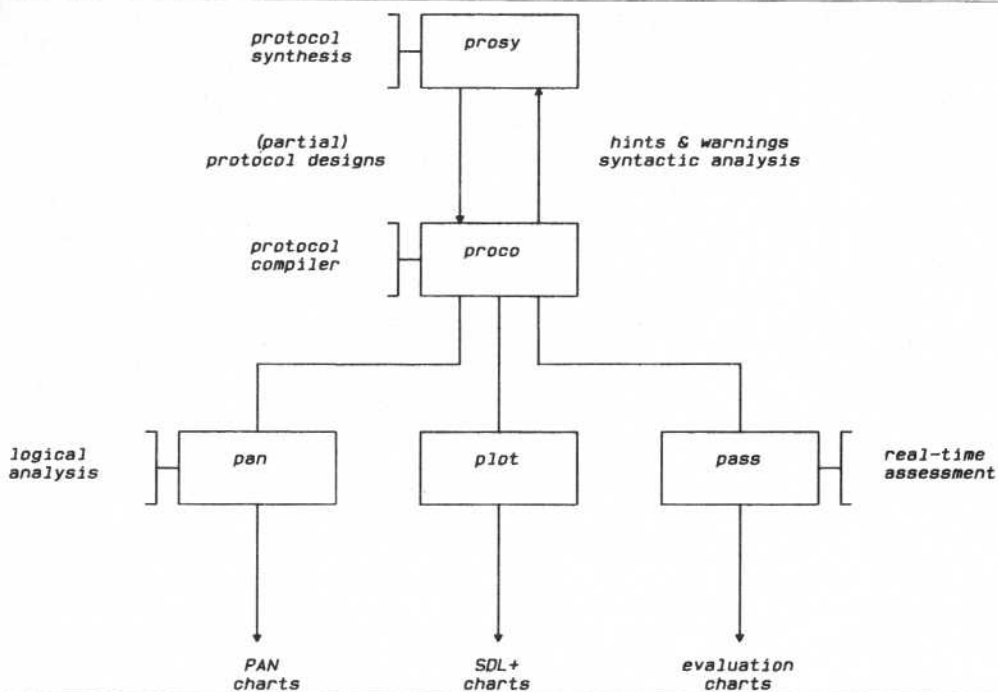
Fig. 2. Software Structure
