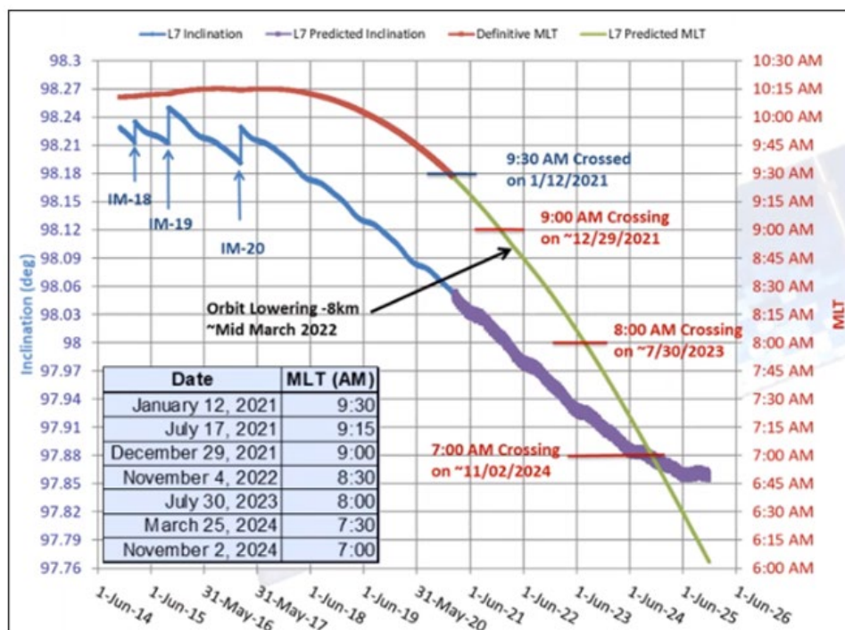
Figure 2-2. Landsat 7 Predicted Drift in Orbital Inclination 2014-2026
