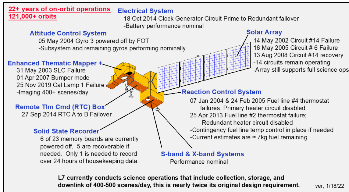
Figure 2-15. Status of Landsat 7 Spacecraft and Subsystems (ca. 2022)
