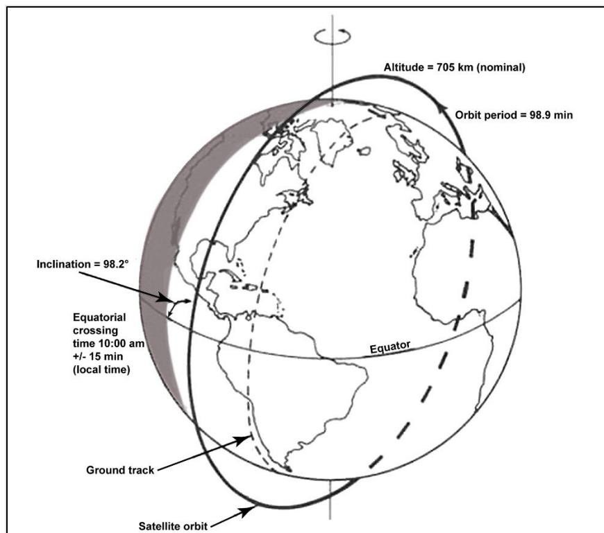
Figure 2-3. Illustration of Landsat 7 Orbit
