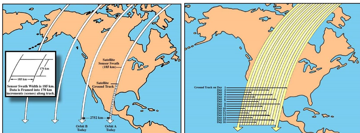
Figure 2-4. ETM+ Swath Separations for Single Day (left) and for Full 16-Day Cycle (right)
