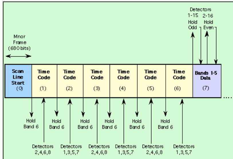
Figure 2-8. Illustration of ETM+ Sample Timing, Format 1
