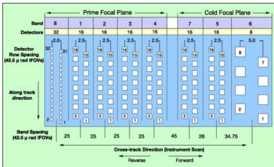
Figure 2-7. Detector Projection at ETM+ Focal Planes
