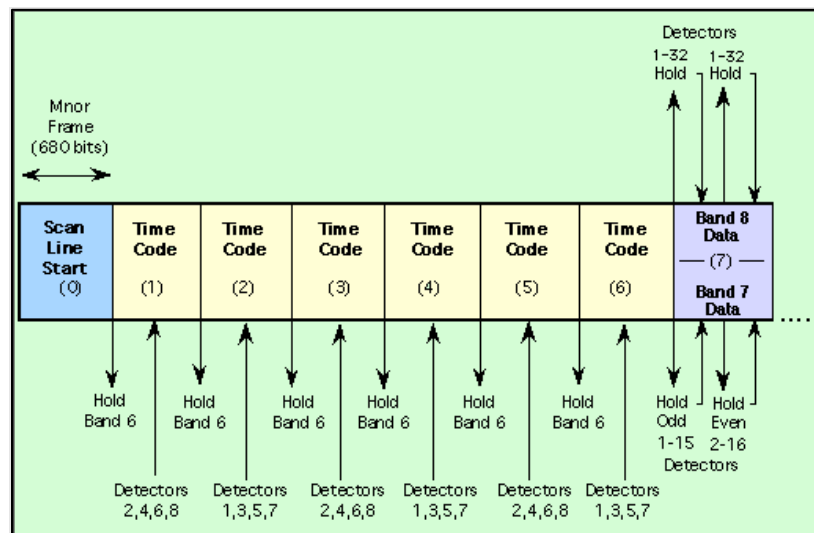
Figure 2-9. Illustration of ETM+ Sample Timing, Format 2
