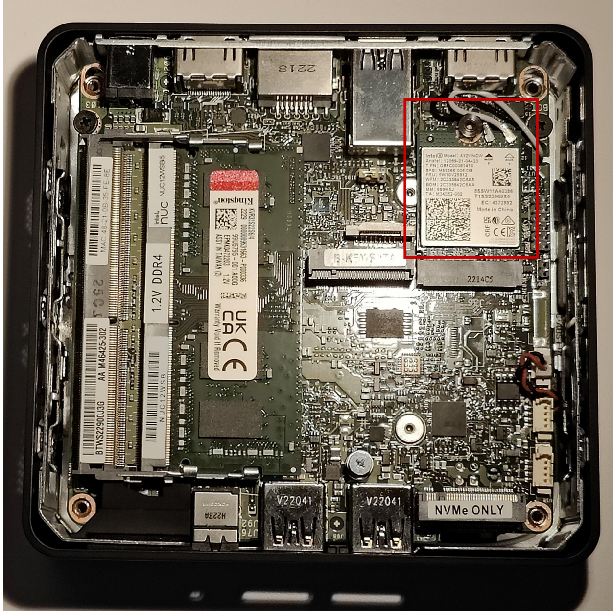
Fig. 4: The location of the wireless card within the NUC12
