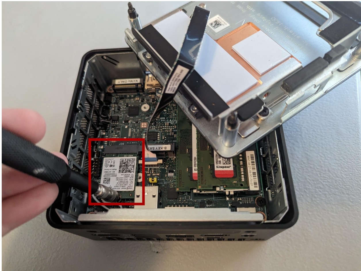
Fig. 3: The location of the wireless card within the NUC13
