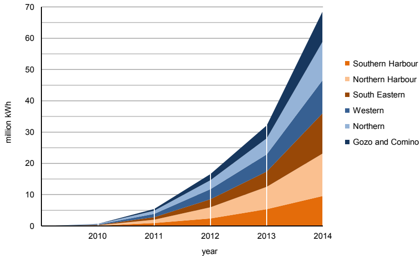
Chart 9.6 Estimated output of connected PVs by district and year
