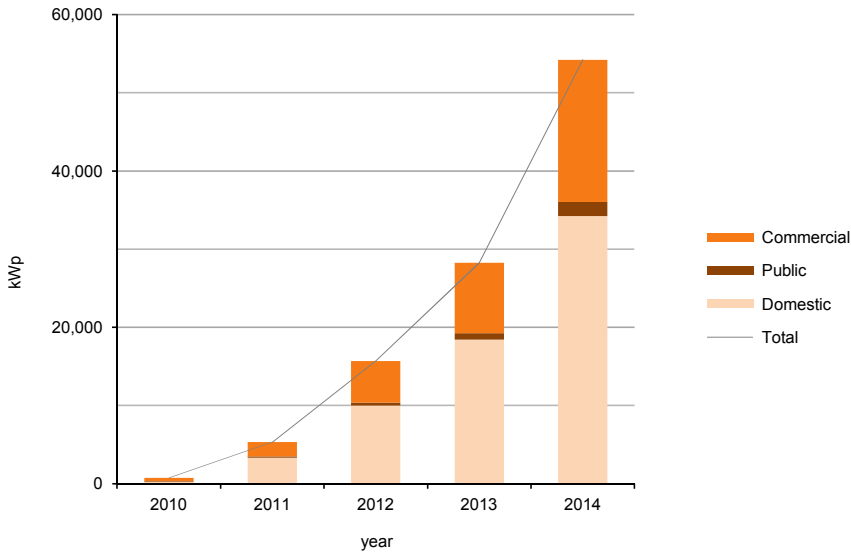
Chart 9.3 Total kWp of connected PVs by sector and year
