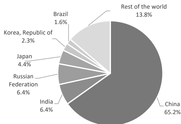
Figure 23: Major coke consuming countries, 2021
