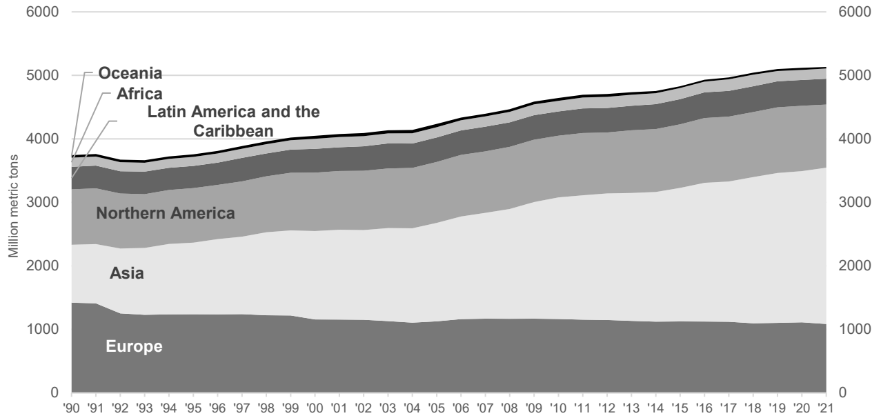
Figure 47: Total refinery distillation capacity by region, 1990-2021
