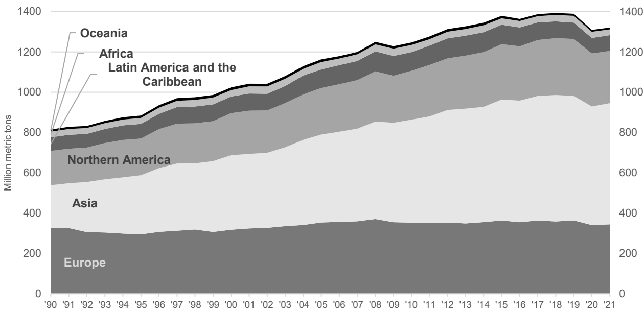
Figure 60: Production of gas oil/diesel oil by region, 1990-2021
