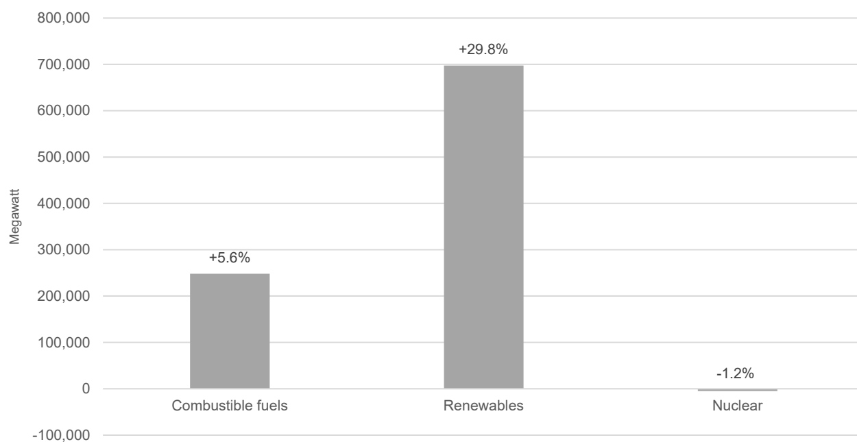
Figure 76: Change in net installed capacity of electricity generating plants* by source, 2018-2021
