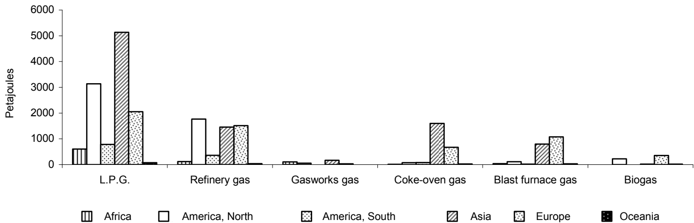
Figure 79: World production of other gases in 2009
