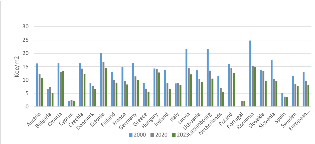
Figure 42: Energy consumption of households for space heating at normal climate in MS, Koe/m 2
