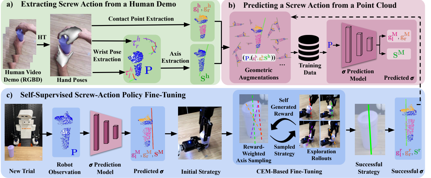
Fig. 2. Overview of SCREW MIMIC. a) Given an RGB-D video of a human performing a bimanual task, we use off-the-shelf hand tracking (HT) models [62, 68] to extract a trajectory of wrist poses \tau^h and grasp contact points (g_l^h, g_r^h) . SCREW MIMIC interprets \tau^h as a screw motion between both hands to estimate screw axis parameters S^h (Sec. IV-A). b) Next, we apply geometric augmentations on the 3D object point cloud to train a PointNet [72] model to estimate screw actions for novel object views (Sec. IV-B). c) Finally, the trained model generates an initial hypothesis that the robot executes and iteratively refines using an autonomously generated reward signal. The successful data point is further used to improve the prediction model (Sec. IV-C).
