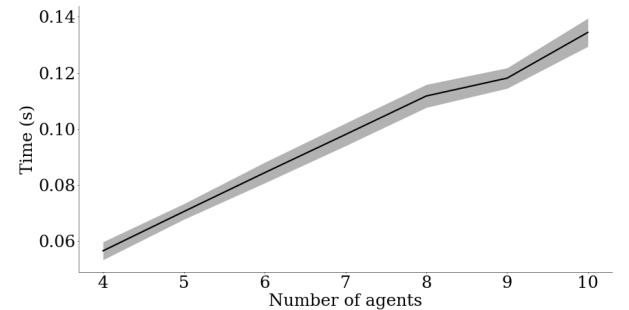
Fig. 7: STP computation time over 100 randomized ATC trials.
