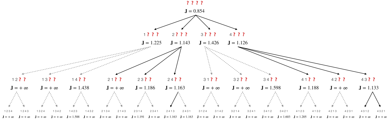
Fig. 15: The full B&P search tree in Figure 4. Dashed grey lines indicate pruned branches. J = +\infty corresponds to cases when STP fails to compute a collision-free LSE.
