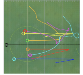
Fig. 10: Case study: quadrotor swarm formation. Each agent's trajectory color represents its priority (warmer is higher). The hollow circles with dashed boundaries represent designated locations of task quadrotors in the half circle to be formed around the leading quadrotor. Compared to the STP policy with a randomized permutation, B&P provides a better trajectory in terms of formation time and reduced extra collision-avoidance maneuvers.
