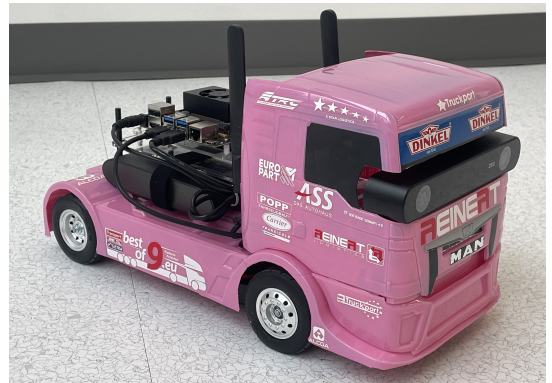
Fig. 12: The autonomous miniature truck platform.
