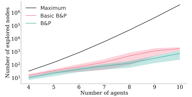
Fig. 6: Number of explored nodes over 100 randomized ATC trials, plotted over the log scale. The solid black line represents the maximum number of explorable nodes.
