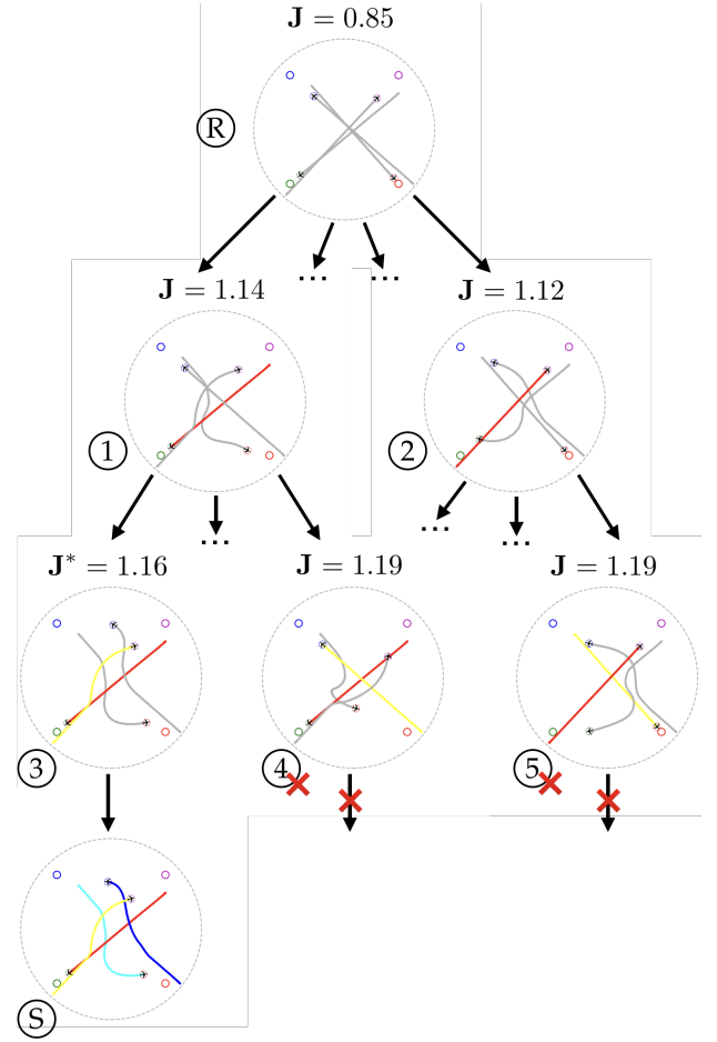
Fig. 4: Illustration of a B&P search tree. Trajectories of unassigned players, who avoid all assigned players, are plotted in grey. In the root node \mathbb{R} , all players are unaware of each other, resulting in a lower bound of the social cost. Players in nodes \mathbb{3} , \mathbb{4} , and \mathbb{5} are collision-free. Unassigned players in those nodes can be given any order of player and there is no need to descend further. Nodes \mathbb{4} and \mathbb{5} are pruned since they produce a higher cost than the feasible solution \mathbb{7} , which turns out to be the optimal solution.
