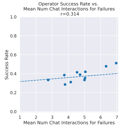
Fig. 7: Correlation of Operator Success Rate and Num Chat Turns until Failures
