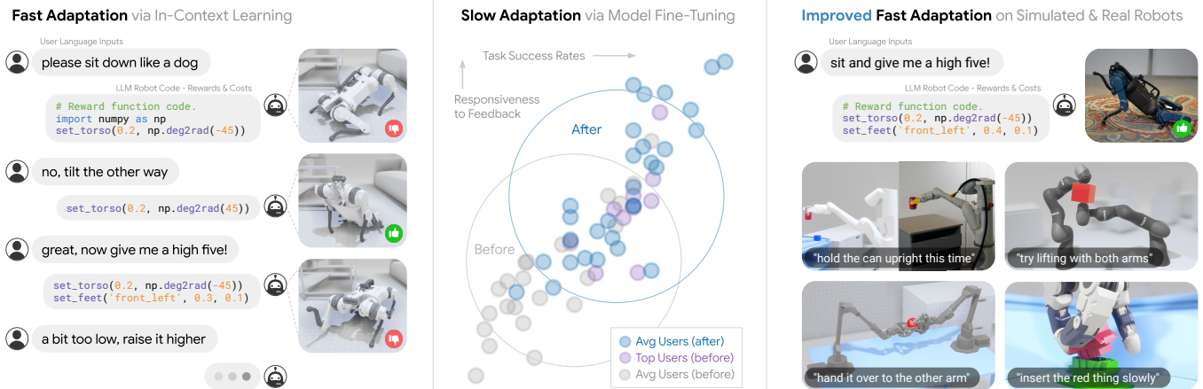
Fig. 1: Code-writing large language models (LLMs) present opportunities for non-experts to teach robots new tasks with language – enabled by fast adaptation via in-context learning (left). In this work, we fine-tune the underlying LLMs to further accelerate fast adaptation and improve their teachability (right). Results with human-robot interactions from non-experts teaching 5 robot embodiments on 78 tasks (gray) show that our framework (middle*) can identify top performing users (purple), and leverage their interactions (only 14% of task coverage) to drive LLM performance improvements for all users (blue) – measured in terms teaching success rates on unseen tasks, responsiveness to user feedback, and number of user corrections. Experiments show that these improvements generalize to new robot embodiments and APIs.
