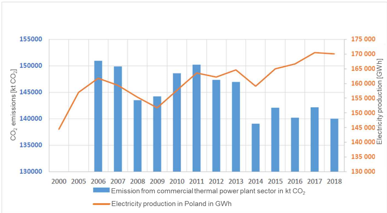
Figure 6. Dynamics of electricity production against GHG emissions from the commercial thermal power plant sector (2006-2018)
