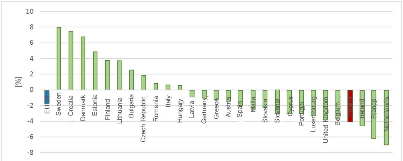
Figure 8. Difference between the share of RES in 2018 and the 2020 target
