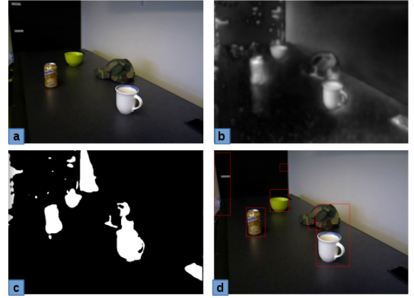
Fig. 2. Steps of object discovery using saliency attention model. a: original image, b: saliency map, c: binary map after thresholding the saliency map, d: bounding boxes around proto-objects
