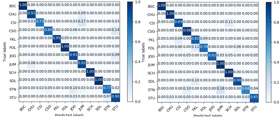
Figure 3: Confusion matrix of best users for both metrics.
