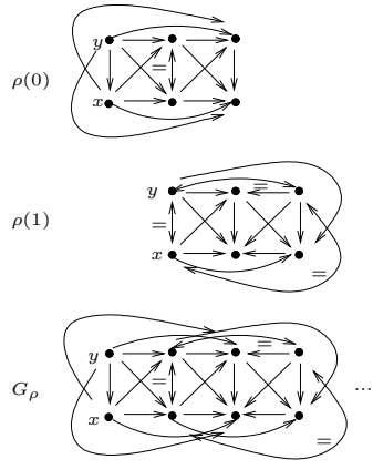
Fig. 1. A 3-frame sequence over the variables \{x, y\}
