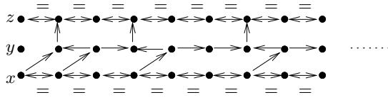
Fig. 2. \rho_{bad}^Z satisfies (C_Z) but does not admit a \mathbb{Z} -valuation sequence.
