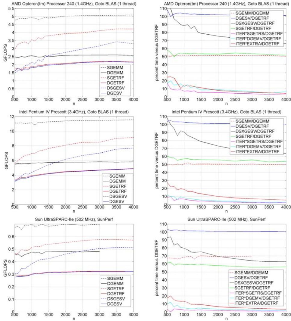
Figure 2: Performance comparison and gain versus DGETRF for DSGESV and its kernels on three different machines.
