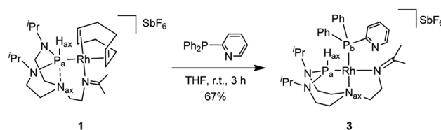
Scheme 3 Preparation of complex 3.
