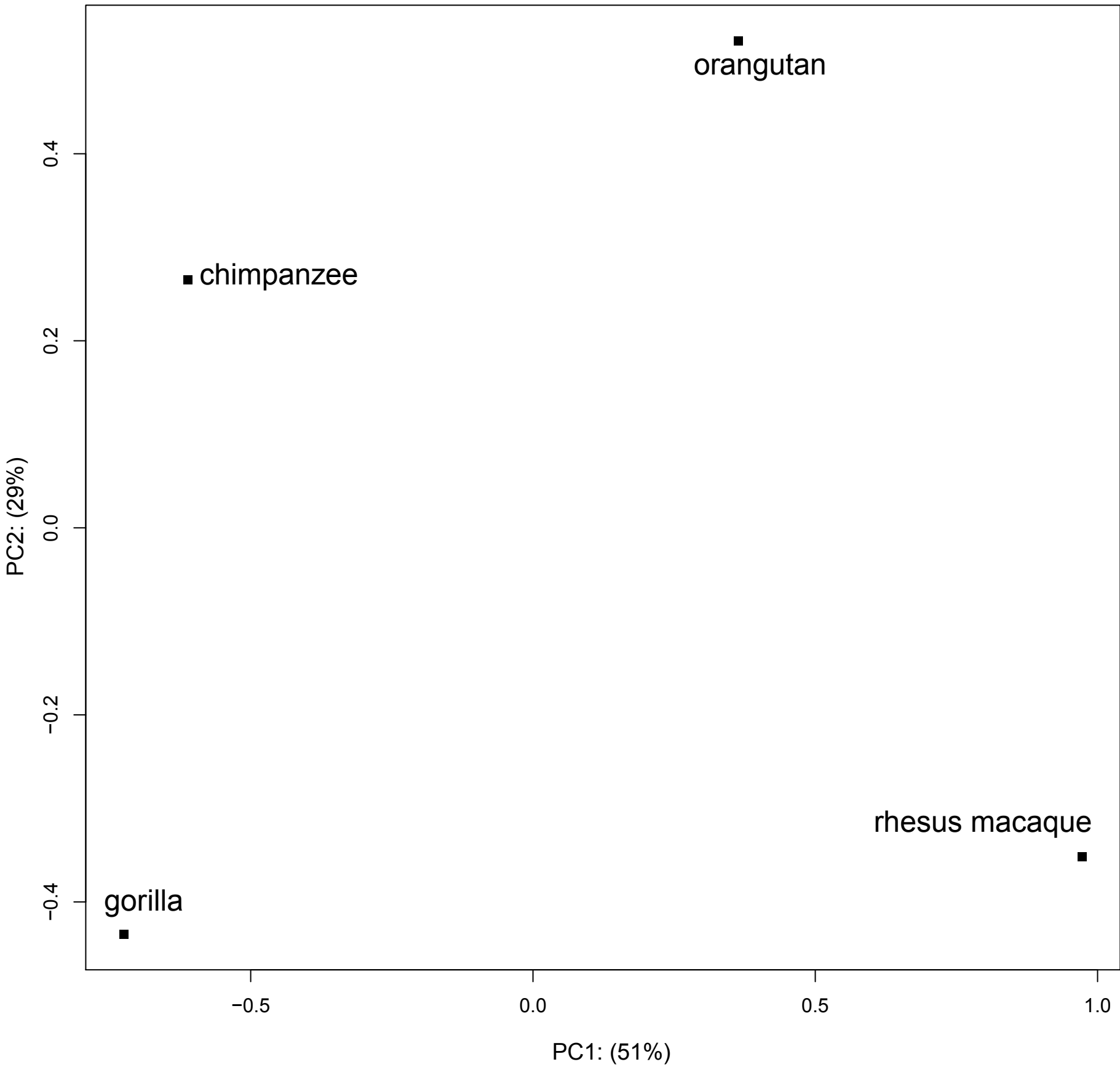
mature sequence
