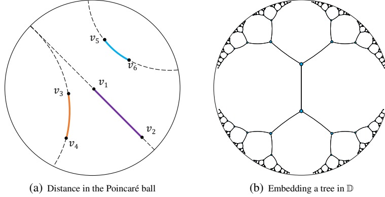
Fig. 2: (a) The colored curves \widehat{v_1v_2} , \widehat{v_3v_4} and \widehat{v_5v_6} indicate the distances between nodes in the Poincaré ball. Geodesics are drawn as dashed curves. It's worth noting that the distance increases exponentially relative to Euclidean distances with the points being closer to the boundary. Best viewed in color. (b) Referred from [20]. It shows an example that a tree (a network with power-law distribution) is embedded into the Poincaré ball.
