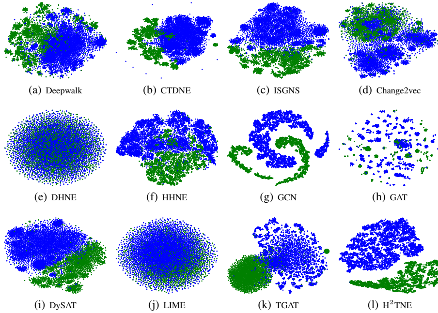
Fig. 5: The visualizations of all baselines and H^2TNE for node classification task in MovieLens. Different colors refer different types of nodes. Best viewed in color.
