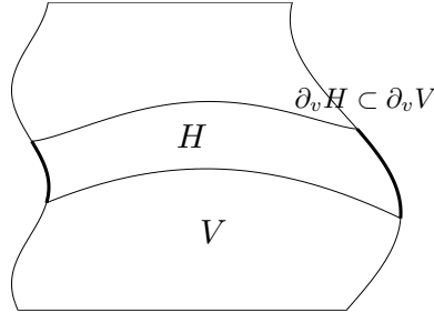
Figure 1. H is bounded by two \mu_h -horizontal curves, each of them linking the two \mu_v -vertical curves composing \partial_v V .
