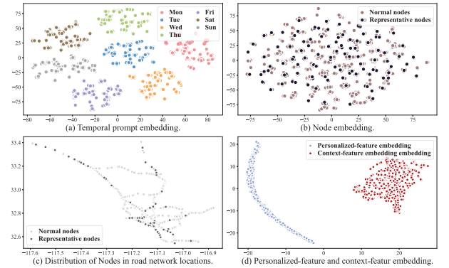
Figure 8: Visualization of various embeddings.
