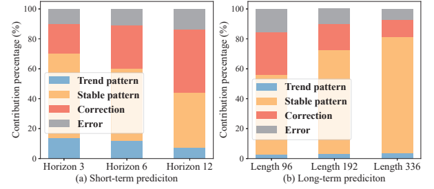
Figure 7: The SHAP values of decomposed components of BiST in SD dataset and (Daily) XXLTraffic dataset.
