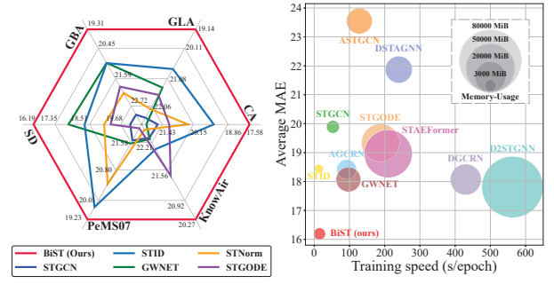
Figure 2: Model performance and efficiency comparison. The left figure illustrates the comparative prediction performance of various models on six datasets. The right figure showcases the training time per epoch and memory usage of each model on LargeST-SD 2019 dataset.
